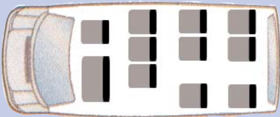
10 or 12 seater conversion for MWB vans
