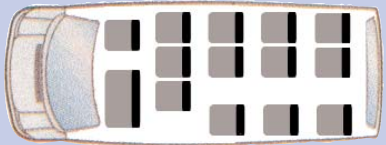
14 or 15 seater conversion for MWB or LWB vans
